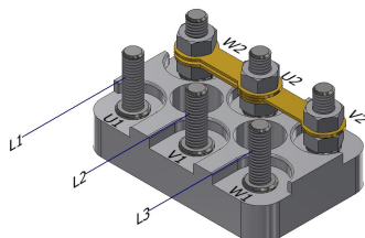
Three – phase connection Star connection
